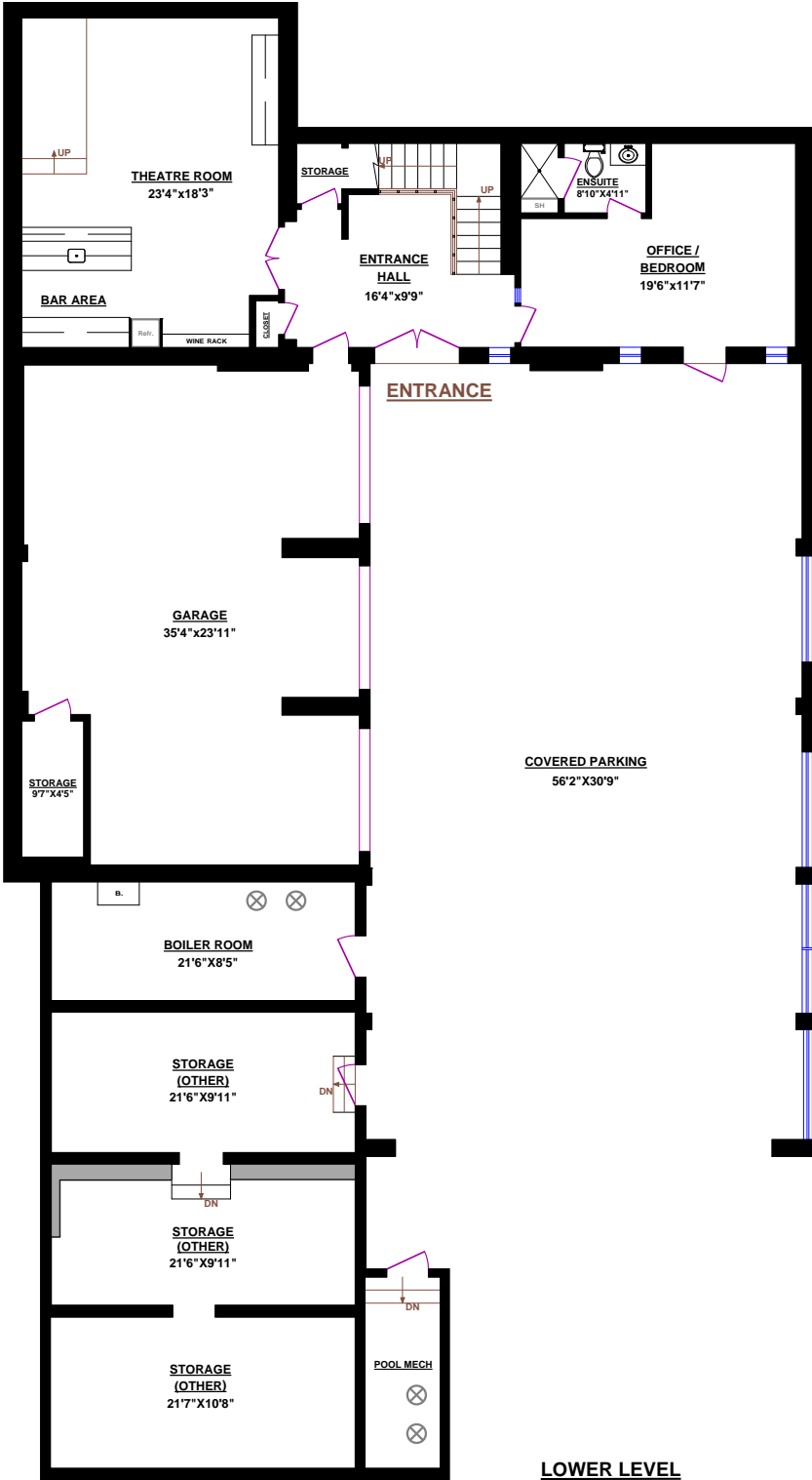
LOWER LEVEL
