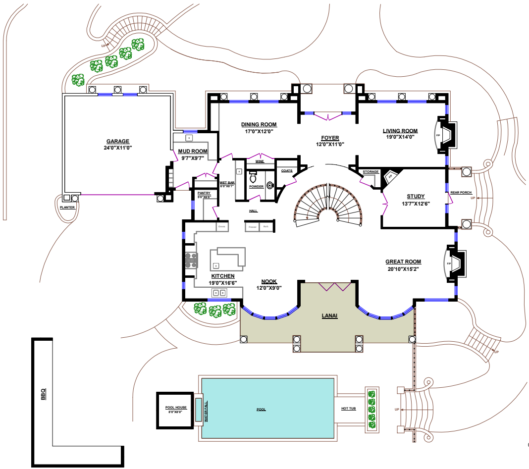
MAIN FLOOR
