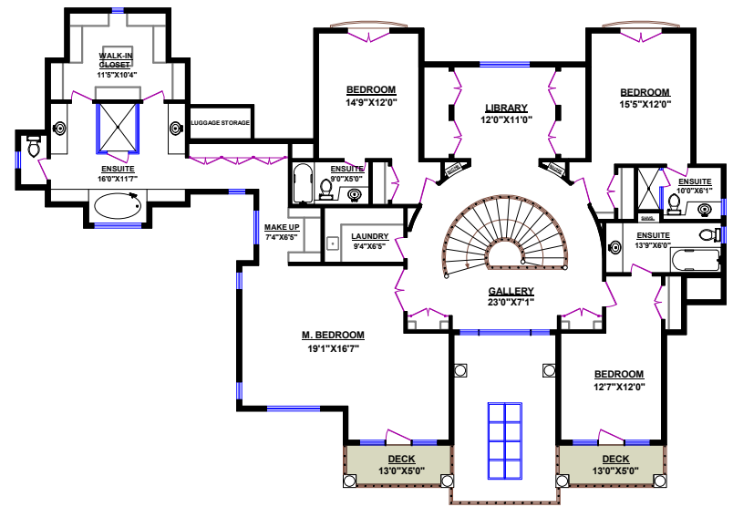
UPPER LEVEL
