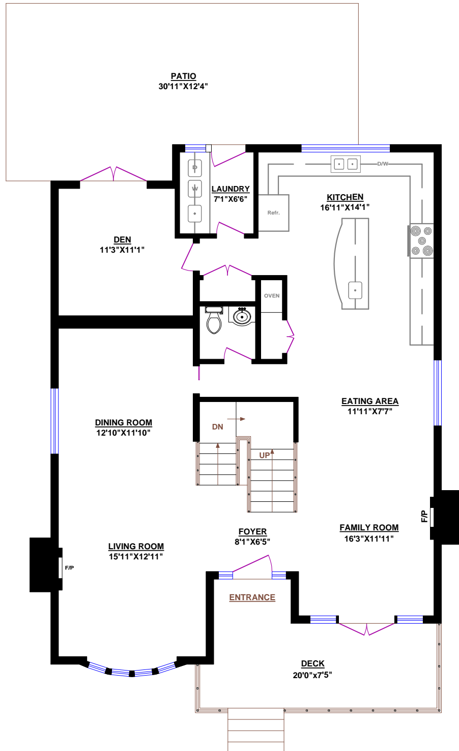
MAIN FLOOR
